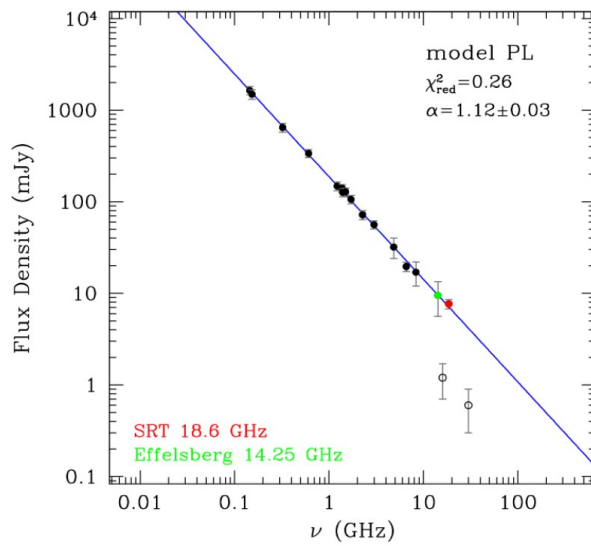
Fig. 5: Spectrum of the total flux density of the Sausage relic. The slope is -1.12 \pm 0.03 (from Loi et al. 2020, arXiv2008.03314).
