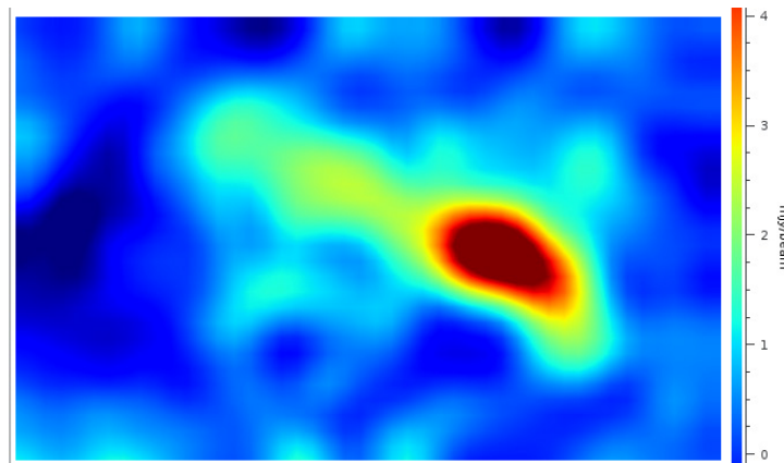
Fig. 4: The Toothbrush relic observed with the Effelsberg telescope at 13-15.5 GHz. The colors show the intensity of the total emission (in units of mJy/beam) (published in Rajpurohit et al. 2020, arXiv2008.02694).
