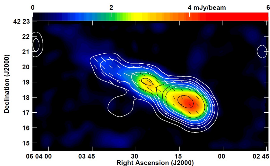
Fig. 2: The radio relic at the edge of the galaxy cluster 1RXS J0603.3+4214, named “Toothbrush”, at a distance of about 900 Mpc. The contour lines show the intensity of the radio emission at 8.35 GHz observed with the Effelsberg telescope, the colors the intensity of the linearly polarized emission (in units of mJy/beam). The lines show the orientation of the ordered magnetic fields (from Kierdorf et al. 2017).
