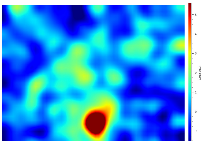
Fig. 3: The Sausage relic observed with the Effelsberg telescope at 13-15.5 GHz. The colors show the intensity of the total emission (in units of mJy/beam) (published in Loi et al. 2020, arXiv2008.03314).
