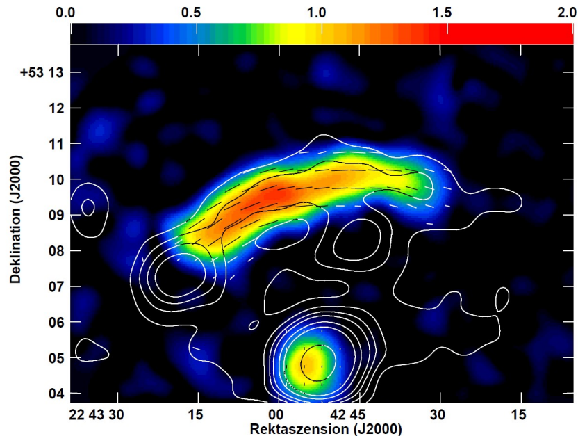
Fig. 1: The radio relic at the edge of the galaxy cluster CIZA J2242+53, named “Sausage”, at a distance of about 800 Mpc. The contour lines show the intensity of the radio emission at 8.35 GHz observed with the Effelsberg telescope, the colors the intensity of the linearly polarized emission (in units of mJy/beam). The lines show the orientation of the ordered magnetic field. The bright source at the bottom of the figure is a radio galaxy that belongs to the same cluster (from Kierdorf et al. 2017).
